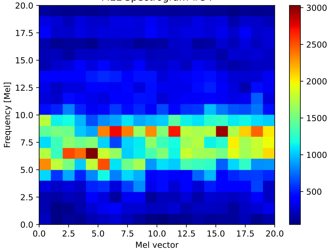
MEL Spectrogram #34
